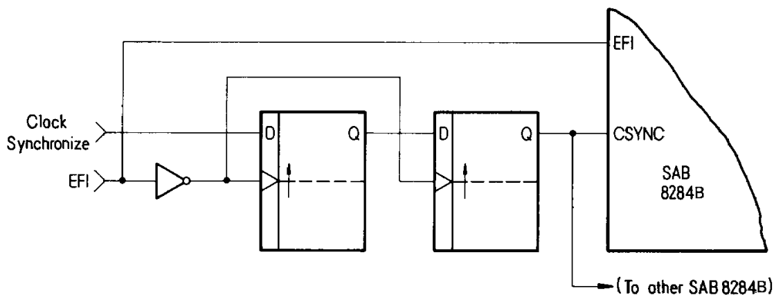
Figure 3 CSYNC Synchronization
