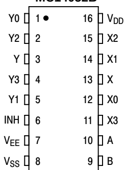
MC14052B
