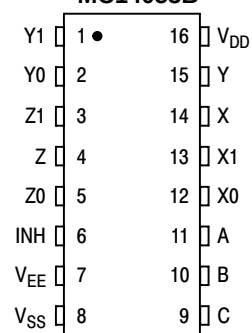
MC14053B
