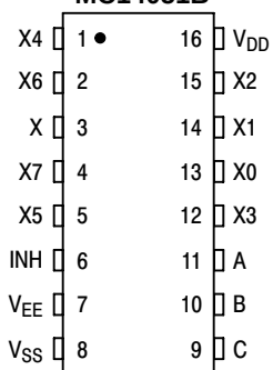
MC14051B
