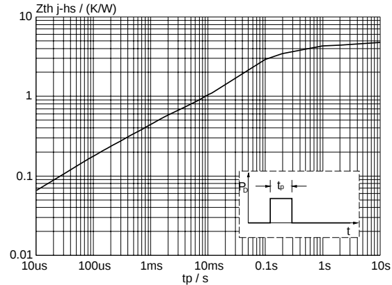
Fig.9. Transient thermal impedance Z_{th} = f(t_p)
