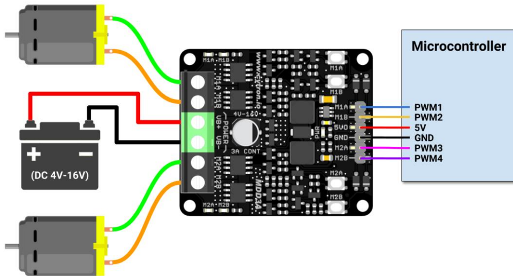
Figure 3: Connection Diagram for Brushed DC Motor
