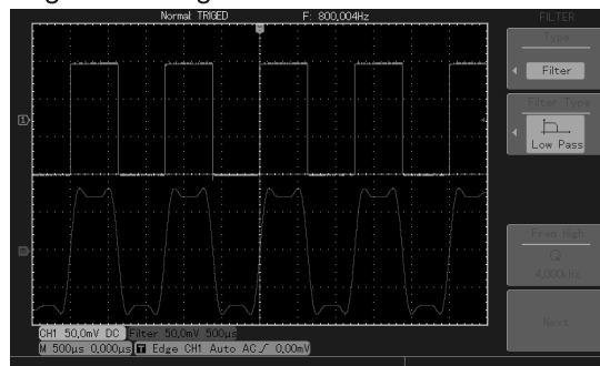
Picture 2-14 Digital filtering
