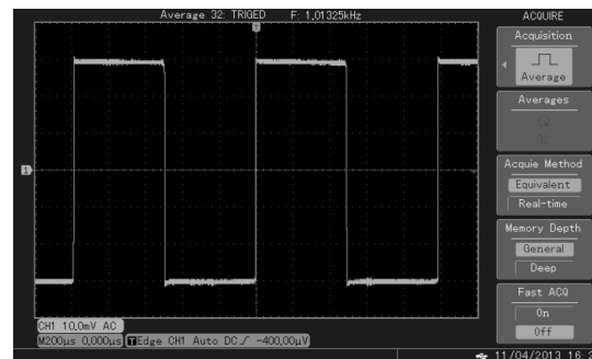
Figure 2— 20 Waveform Display Using 32-times Average Mode
