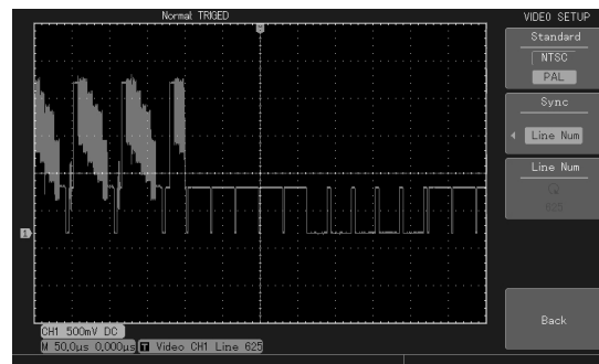
Figure 3-33 Video Horizontal Trigger
