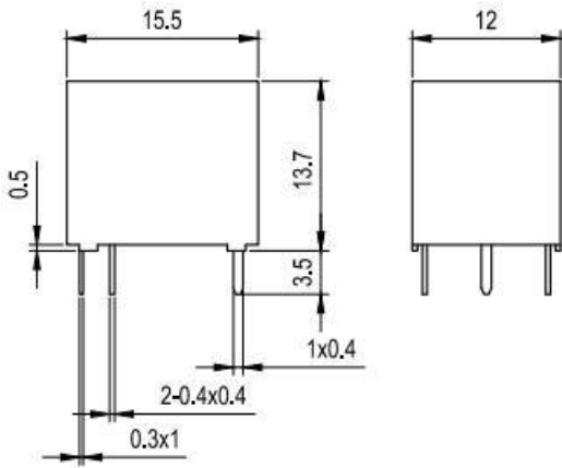
1C Outline Dimensions
