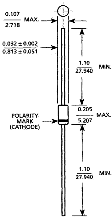
All Dimensions in \frac{\text{Inch}}{\text{m.m.}}
