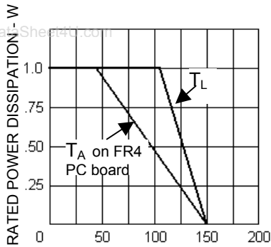
T_L , LEAD TEMP. ( ^{\circ}\text{C} ) 3/8" from body or T_A on FR4 PC Board
