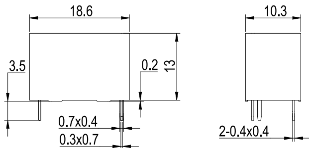
1A4 Outline Dimensions
