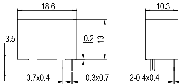
1A2 Outline Dimensions
