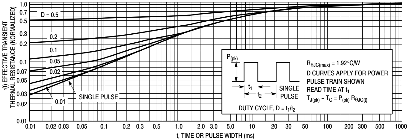
Figure 4. Thermal Response
