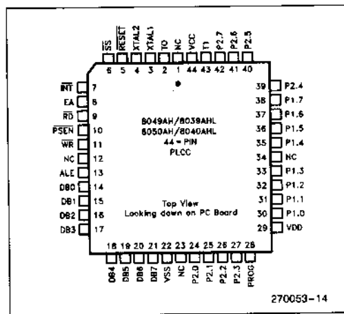
Figure 4. Pad Configuration
