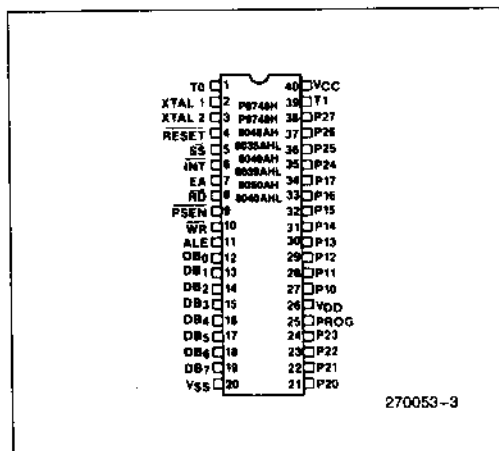
Figure 3. Pin Configuration
