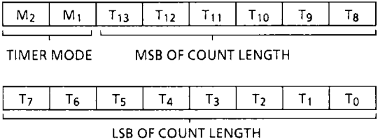
Figure 6.3 Timer Format
