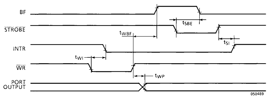
Figure 8.6 STROBED OUTPUT MODE
