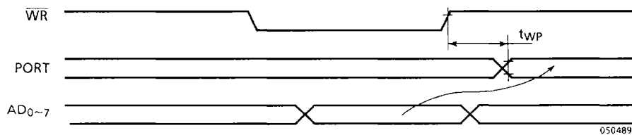
Figure 8.4 BASIC OUTPUT MODE
