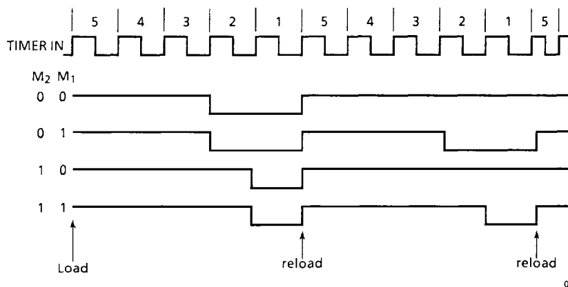
Figure 6.3 Asymmetrical Square-Wave Output resulting from Count 5
