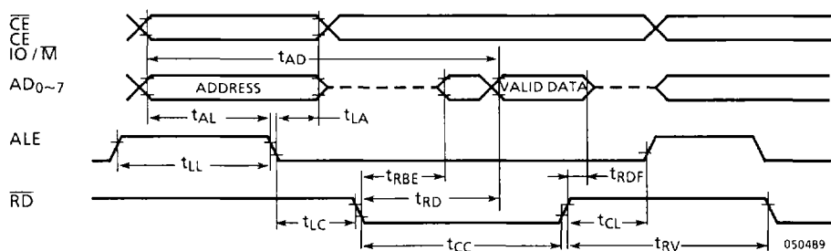
Figure 8.1 READ CYCLE
