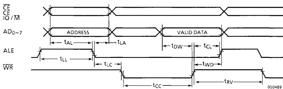
Figure 8.2 WRITE CYCLE
