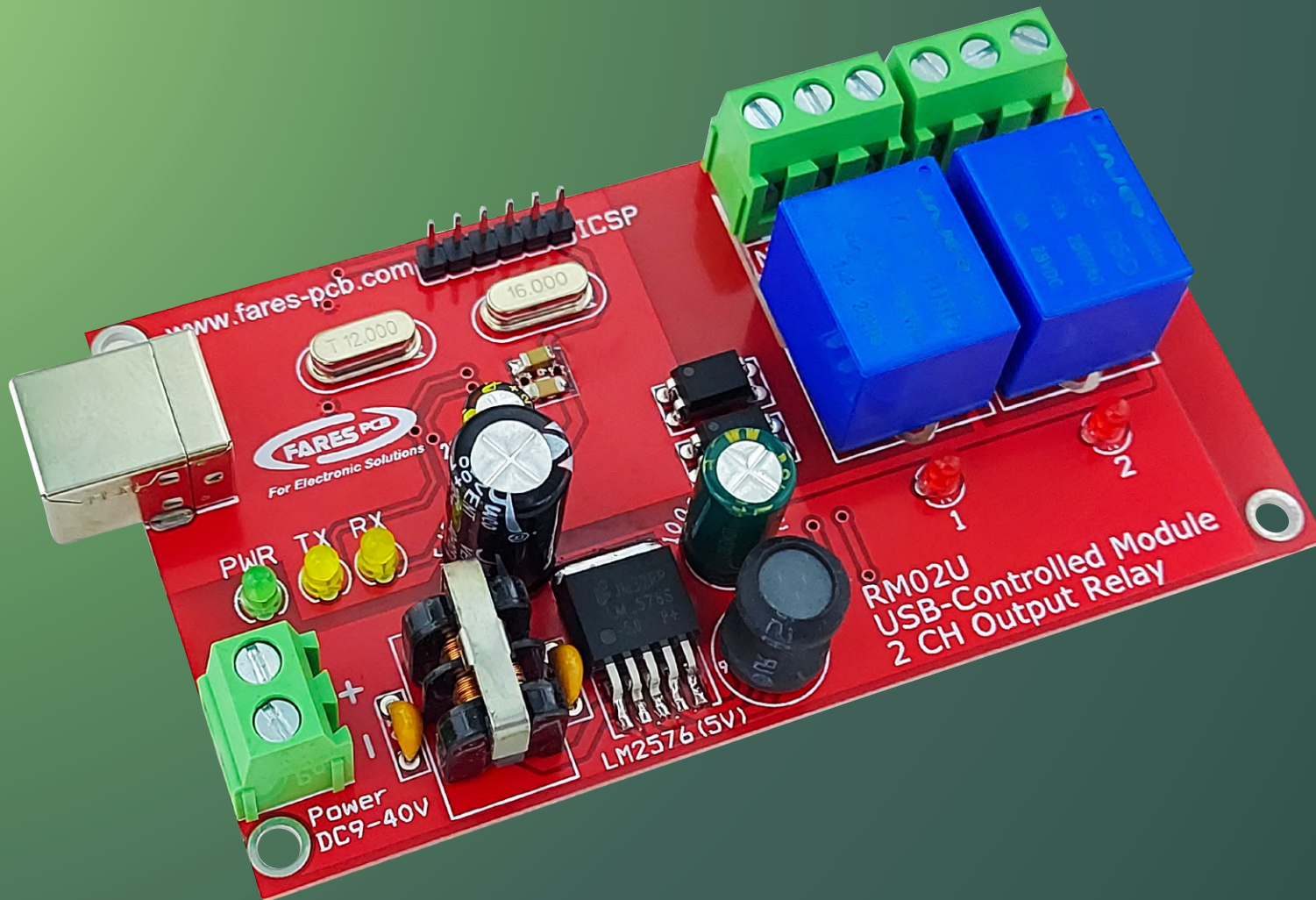
2-Channel USB-Controlled Relay Module
