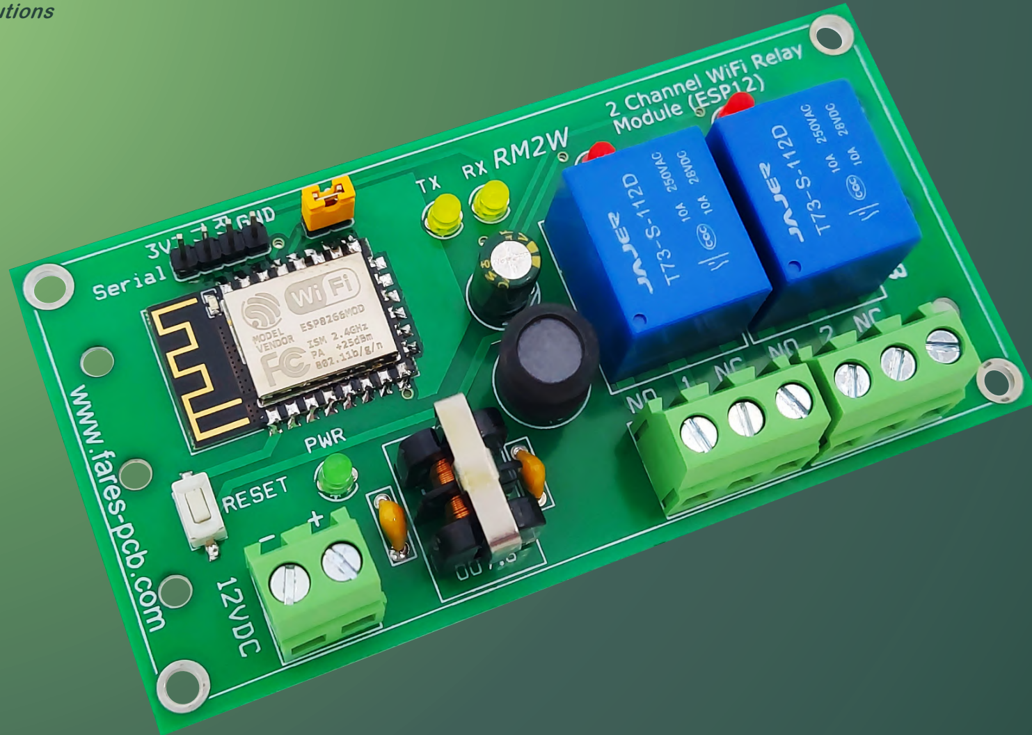
2-Channel Wi-Fi Relay Module
