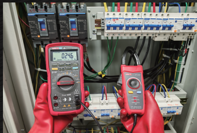
Power distribution box Current measurement
