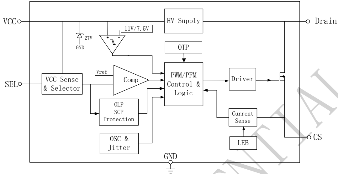
Figure 4. BP2522X Internal Block Diagram
