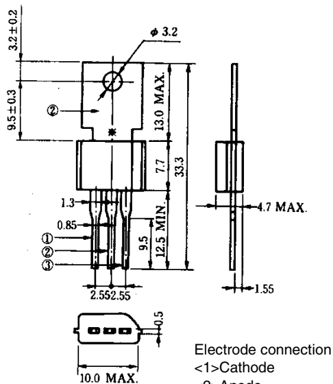
PACKAGE DRAWING (UNIT: mm)
