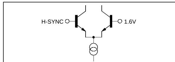
Figure 6 : Input Structure
