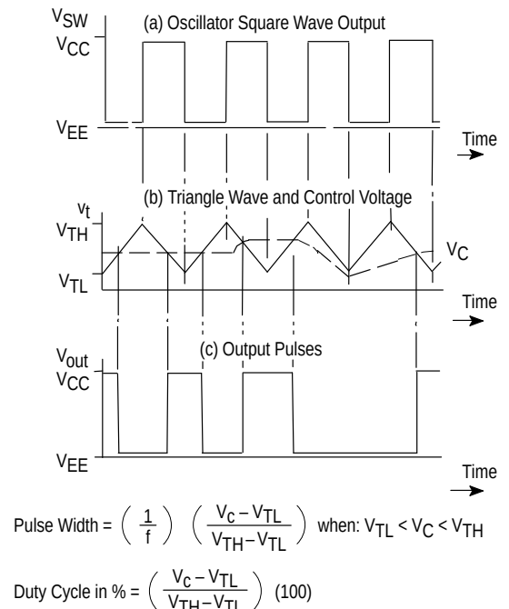
Figure 11. Pulse Width Modulator Schematic and Waveforms
