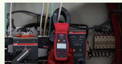
Measurement of AC Current in Distribution Cabinets
